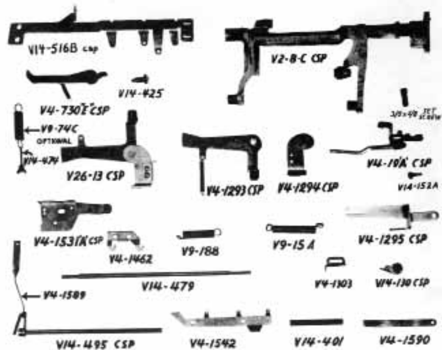
FRAME ATTACHMENTS - REAR OF MECHANISM
